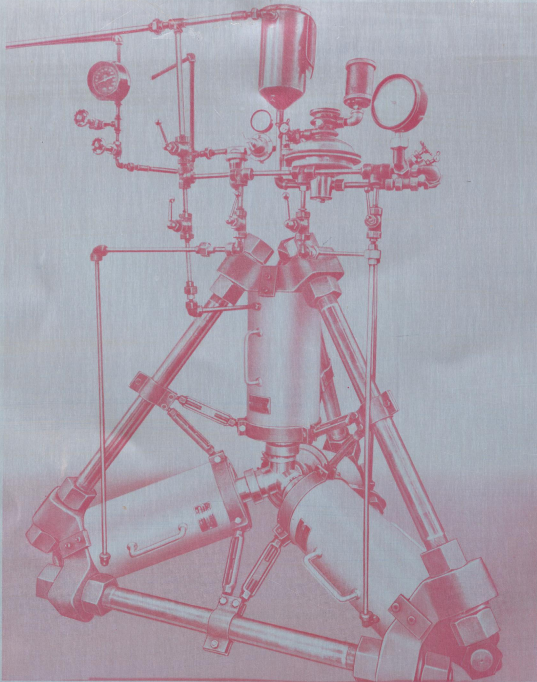
TETRAHEDRAL ANVIL APPARATUS
